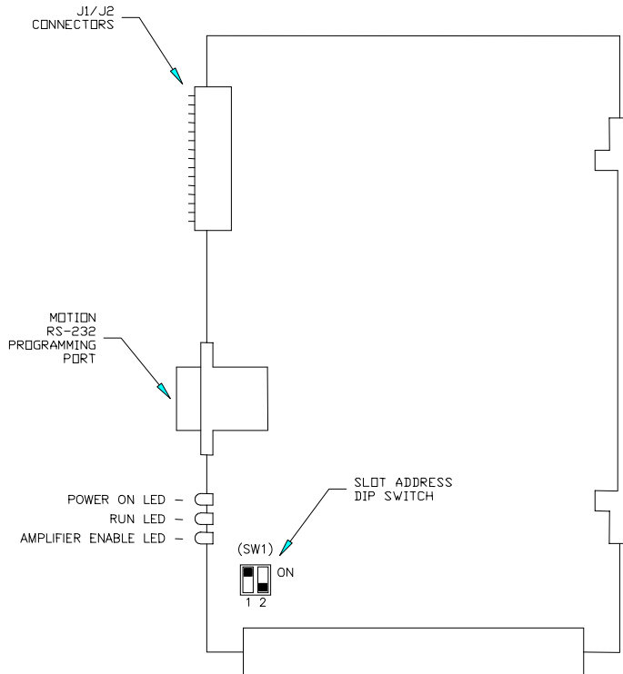
Figure 2 S4520-ENC Board Outline
