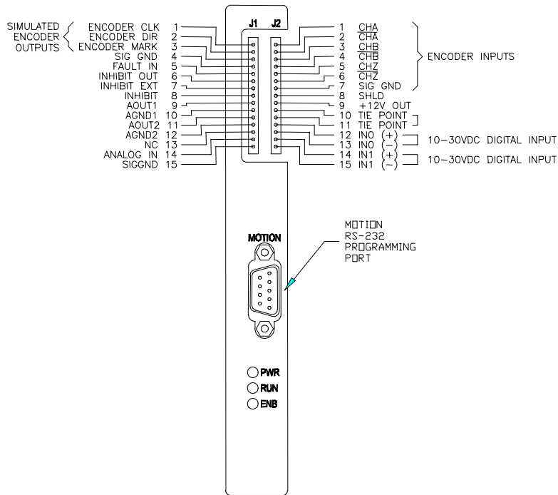
Figure 1 S4520-ENC Faceplate
